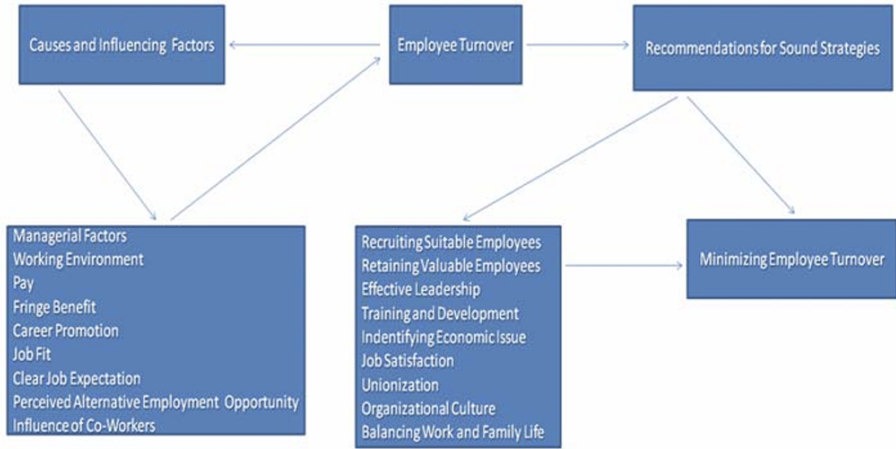
Fig. 1. Conceptual framework
