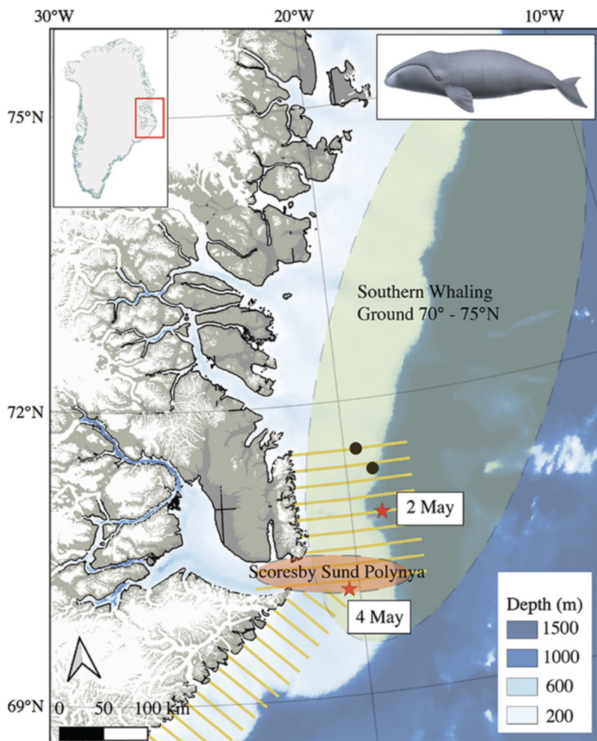
Fig. 1 The locations of bowhead whale sightings during the survey in 2022: two bowhead whale mother-calf pairs (red stars) and two additional adults (black dots). The mother-calf pair observations were made on 2 and 4 May, about 100 km apart, qualifying them as observations of unique individuals. The yellow stripes indicate the approximate location of the Southern Whaling Ground utilized between the early 1600 and 1900s (Allen & Keay 2006). The yellow-shaded oval marks the general area of the Scoresby Sund Polynya. (Illustration of the bowhead whale calf by U. Gorter.)
